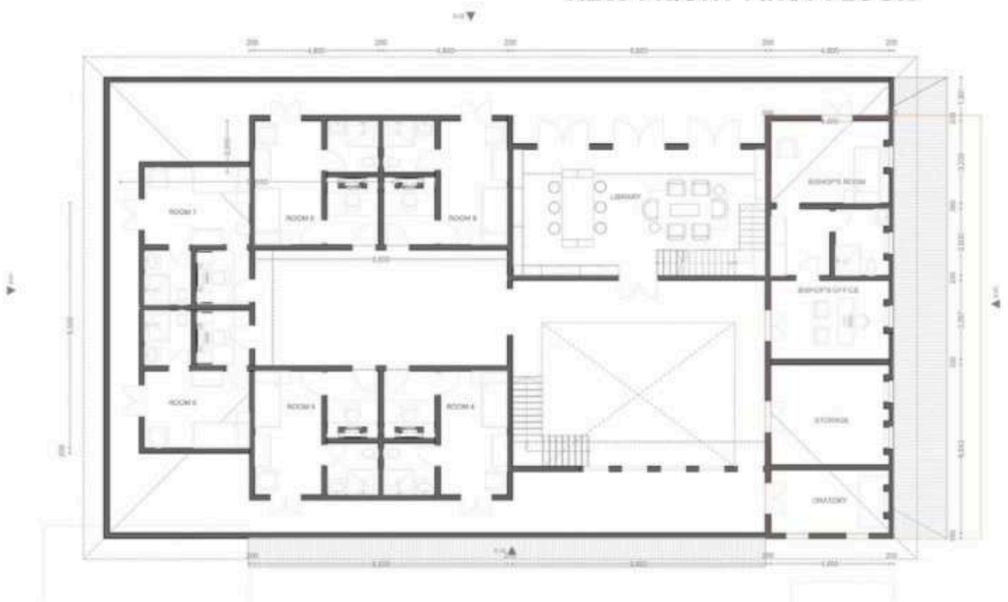
NEW PRIORY FIRST FLOOR
