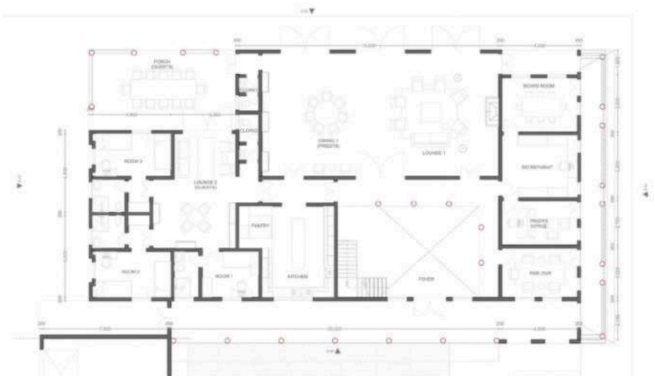
NEW PRIORY GROUND FLOOR
